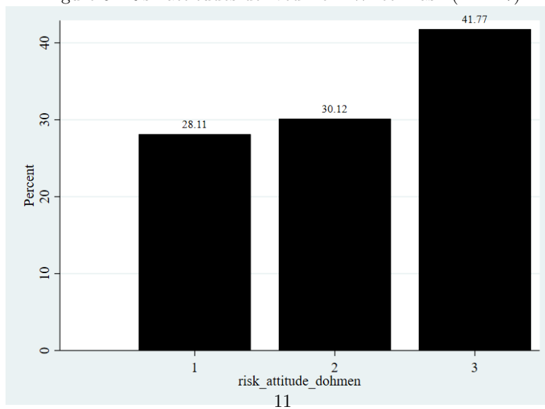
Figure 7: Risk attitudes derived from Dohmen Question (N=247)
